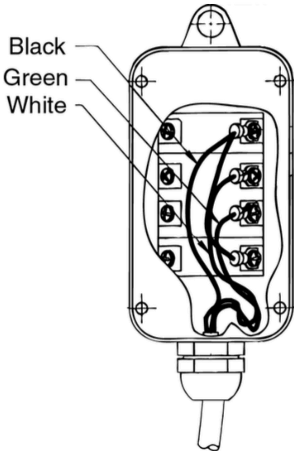
3 - Wire Cord (3 Way) Terminal Connections
